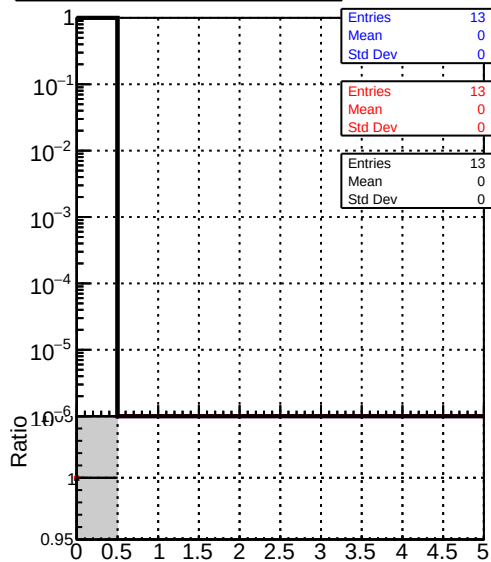
mean hits DQM_V0001_R000000001_Global_CMSSW_100ti DQM_V0001_R000000001_Global_CMSSW_100timeHPTT DQM_V0001_R000000001_Global_CMSSW_100timePLa
