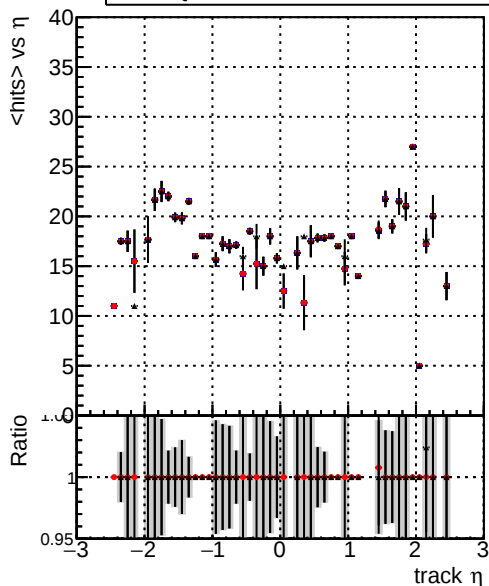
mean hits vs \eta Legend: DQM_V0001_R000000001_Global_CMSSW_100ti (blue), DQM_V0001_R000000001_Global_CMSSW_100timeHPTT (red), DQM_V0001_R000000001_Global_CMSSW_100timePLa (black)
