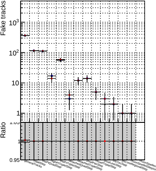
Number DQM_V0001_R000000001_Global_CMSSW_100timeHP1 DQM_V0001_R000000001_Global_CMSSW_100timePLa
