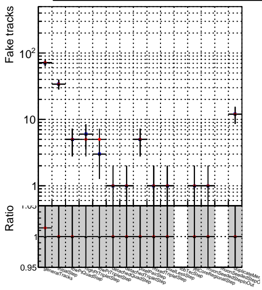
Number
