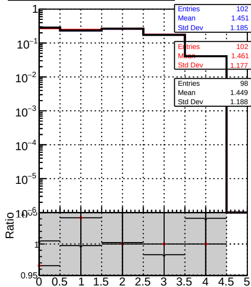
mean hit DQM_V0001_R000000001_Global_CMSSW_100ti DQM_V0001_R000000001_Global_CMSSW_100timeHPTT DQM_V0001_R000000001_Global_CMSSW_100timePLa
