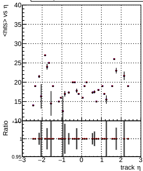
mean hit Legend: - DQM_V0001_R000000001_Global_CMSSW_100ti (blue line) - DQM_V0001_R000000001_Global_CMSSW_100timeHPTT (red line) - DQM_V0001_R000000001_Global_CMSSW_100timePLa (black line)
