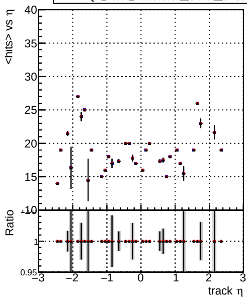
mean hit Legend: DQM_V0001_R000000001_Global_CMSSW_100ti (blue), DQM_V0001_R000000001_Global_CMSSW_100timeHPTT (red), DQM_V0001_R000000001_Global_CMSSW_100timePLa (black)
