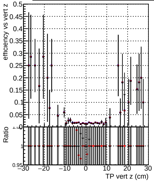
Efficiency vs. sim PV z —●— DQM_V0001_R0000000001_Global_CMSSW_100ti —●— DQM_V0001_R0000000001_Global_CMSSW_100timeHPTT —●— DQM_V0001_R0000000001_Global_CMSSW_100timePLa
