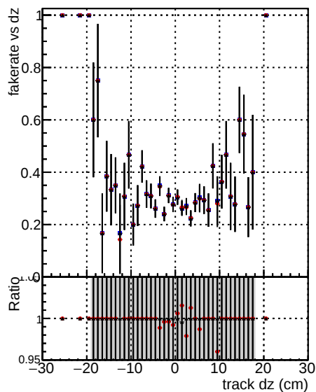
Fake rate vs d d DOM V0001 R0000000001 Global CMSSW 100ti DOM V0001 R0000000001 Global CMSSW 100timeHPTT DOM V0001 R0000000001 Global CMSSW 100timePLa 0 0.8 0.8 0.8 1 0.05 0.05 0.05 2 0.02 0.02 0.02 3 0.01 0.01 0.01 4 0.01 0.01 0.01 5 0.01 0.01 0.01 6 0.01 0.01 0.01 7 0.01 0.01 0.01 8 0.01 0.01 0.01 9 0.01 0.01 0.01 10 0.01 0.01 0.01
