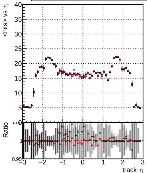
mean hits — DQM_V0001_R000000001_Global_CMSSW_100ti — DQM_V0001_R000000001_Global_CMSSW_100timeHPTT — DQM_V0001_R000000001_Global_CMSSW_100timePLa
