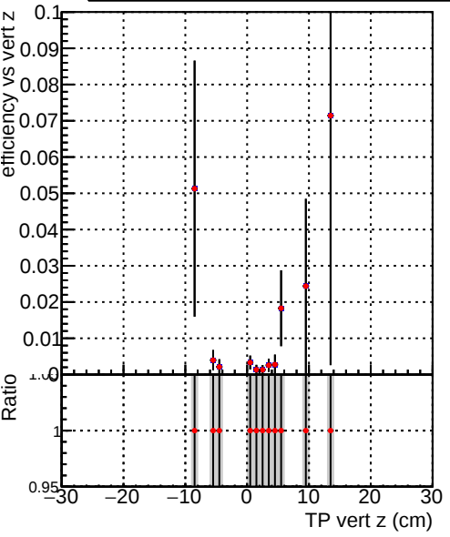
Efficiency vs vertpos Legend: DQM_V0001_R0000000001_Global_mkFit_baseline1 DQM_V0001_R0000000001_Global_mkFit_batch1
