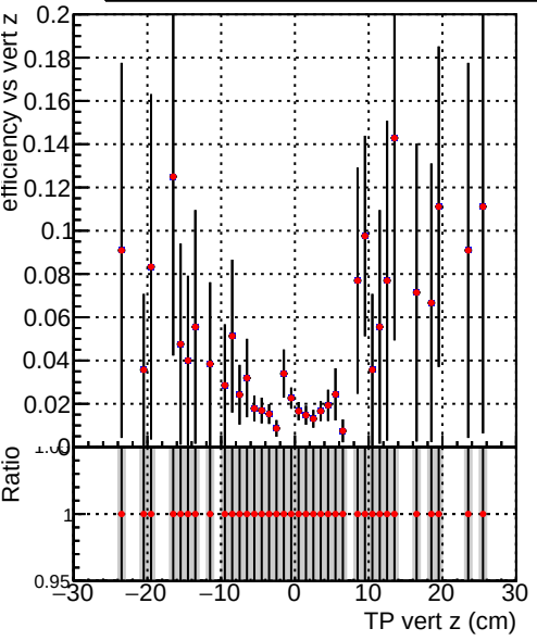
Efficiency vs TP vert z (cm) Legend: DQM_V0001_R0000000001_Global_mkFit_baseline1 DQM_V0001_R0000000001_Global_mkFit_batch1
