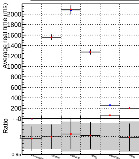
Average —●— DOM V0001 R0000000001 Global mkFit batch1
