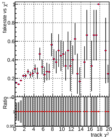
Fake rate vs. Legend Global mkFit baseline1 Blue star DQM_V0001_R0000000001 Red star DQM_V0001_R0000000001 mkFit batch1
