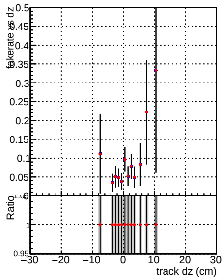
Fake rate vs dz —•— DQM_V0001_R0000000001_Global_mkFit_baseline1 —•— DQM_V0001_R0000000001_Global_mkFit_batch1
