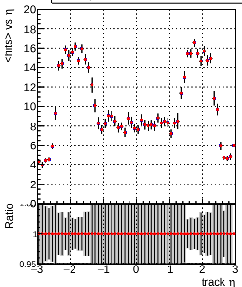
— DQM_V0001_R000000001_Global_mkFit_baseline1 — DQM_V0001_R000000001_Global_mkFit_batch1
