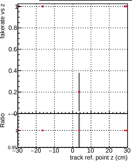
DQM_V0001_R000000001_Global_mkFit_baseline1 DQM_V0001_R000000001_Global_mkFit_batch1
