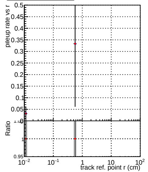
DQM_V0001_R000000001_Global_mkFit_baseline1 DQM_V0001_R000000001_Global_mkFit_batch1
