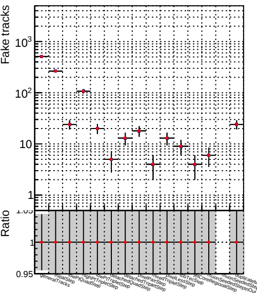
Number —●— DQM_V0001_R000000001_Global_mkFit_batch1
