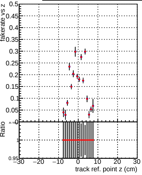
Fake rate vs verpos —●— DQM_V0001_R000000001_Global_mkFit_baseline1 —◆— DQM_V0001_R000000001_Global_mkFit_batch1
