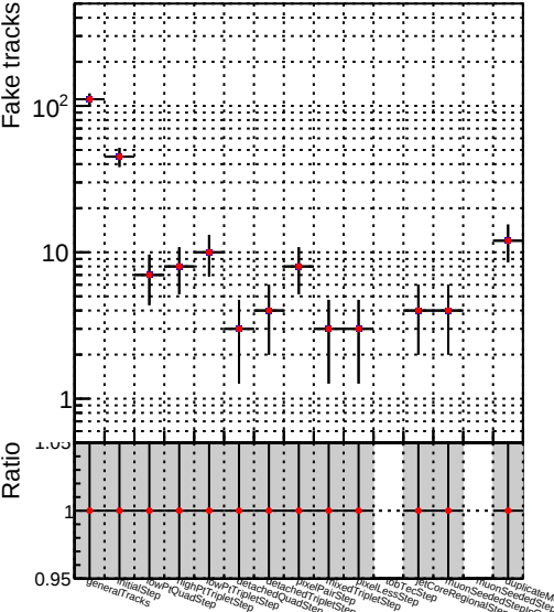
Number —●— DQM_V0001_R000000001_Global_mkFit_batch1
