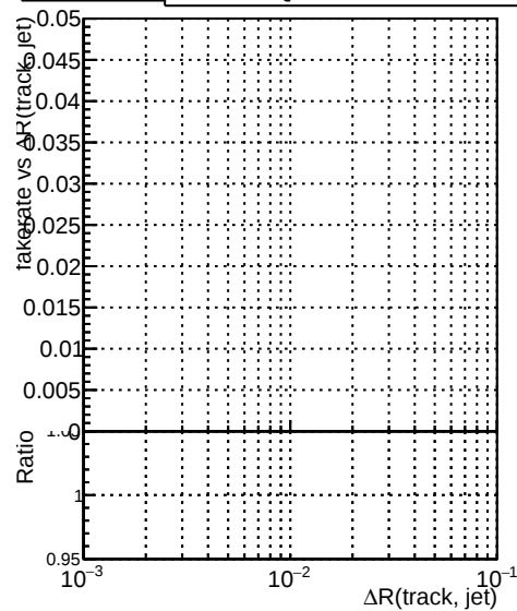
—•— DQM_V0001_R000000001_Global_mkFit_baseline1 —•— DQM_V0001_R000000001_Global_mkFit_batch1
