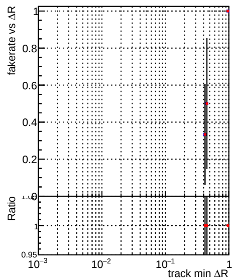
—•— DQM_V0001_R000000001_Global_mkFit_baseline1 —•— DQM_V0001_R000000001_Global_mkFit_batch1
