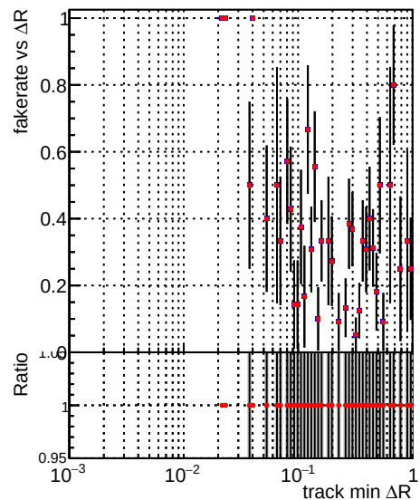
—•— DQM_V0001_R000000001_Global_mkFit_baseline1 —•— DQM_V0001_R000000001_Global_mkFit_batch1
