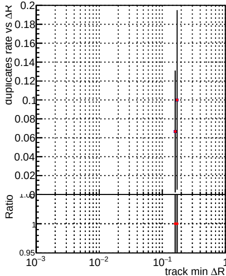
—•— DQM_V0001_R000000001_Global_mkFit_baseline1 —•— DQM_V0001_R000000001_Global_mkFit_batch1
