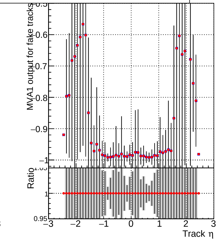
MVA1 of non-associated tracks (recoToSim) vs. track \eta
