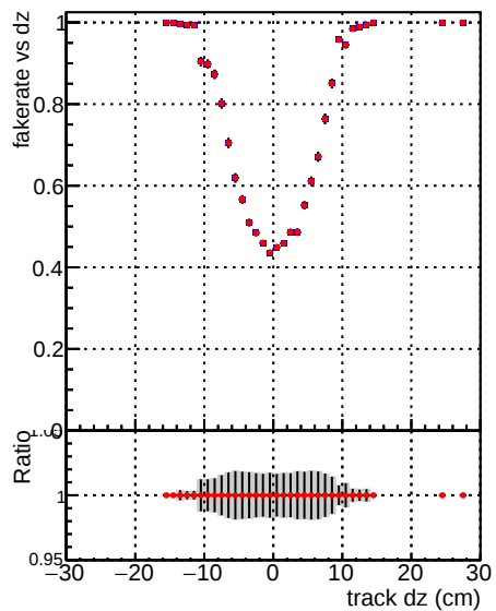
Fake rate vs dz —●— DQM_V0001_R0000000001_Global_mkFit_baseline1 —●— DQM_V0001_R0000000001_Global_mkFit_batch1
