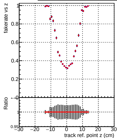
—●— DQM_V0001_R000000001_Global_mkFit_baseline1 —◆— DQM_V0001_R000000001_Global_mkFit_batch1
