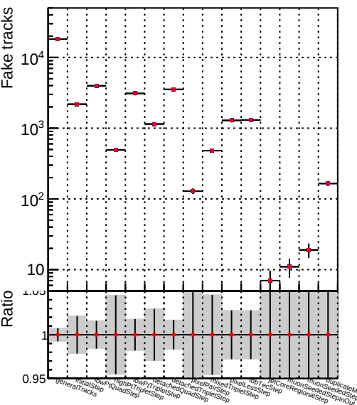
Number —●— DQM_V0001_R000000001_Global_mkFit_batch1
