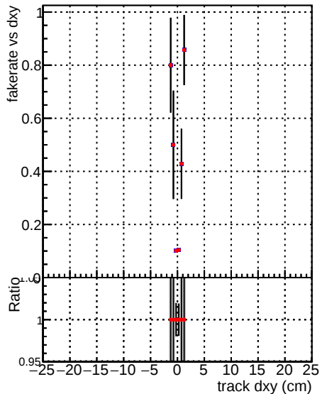
—•— DQM_V0001_R0000000001_Global_mkFit_baseline1 —•— DQM_V0001_R0000000001_Global_mkFit_batch1
