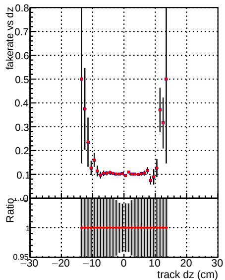
—•— DQM_V0001_R0000000001_Global_mkFit_baseline1 —•— DQM_V0001_R0000000001_Global_mkFit_batch1
