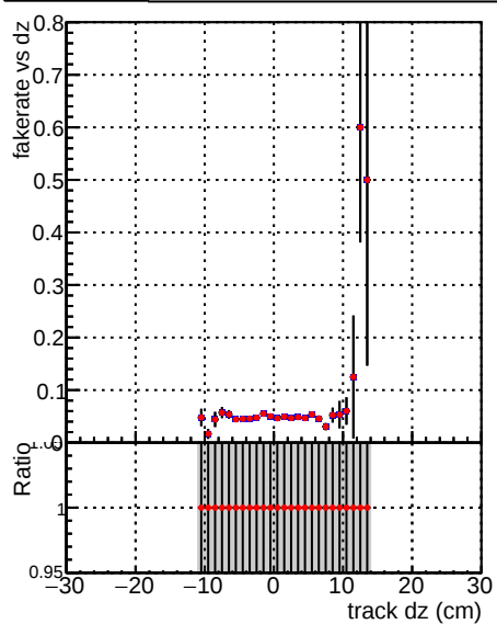
—•— DQM_V0001_R0000000001_Global_mkFit_baseline1 —•— DQM_V0001_R0000000001_Global_mkFit_batch1
