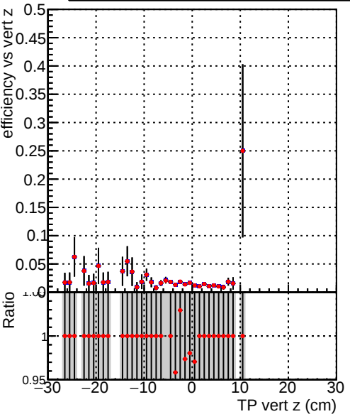
Efficiency vs vertpos Legend: DQM_TT_originalCustomized DQM_TT_nocutCustomized
