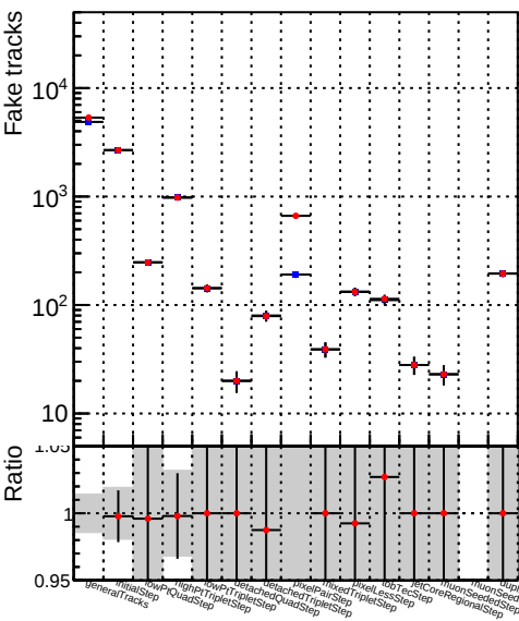
Number —●— DQM_TT_nocutCustomized
