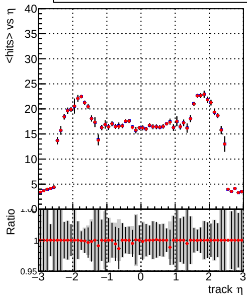
mean hit — DQM_TT__originalCustomized — DQM_TT__nocutCustomized
