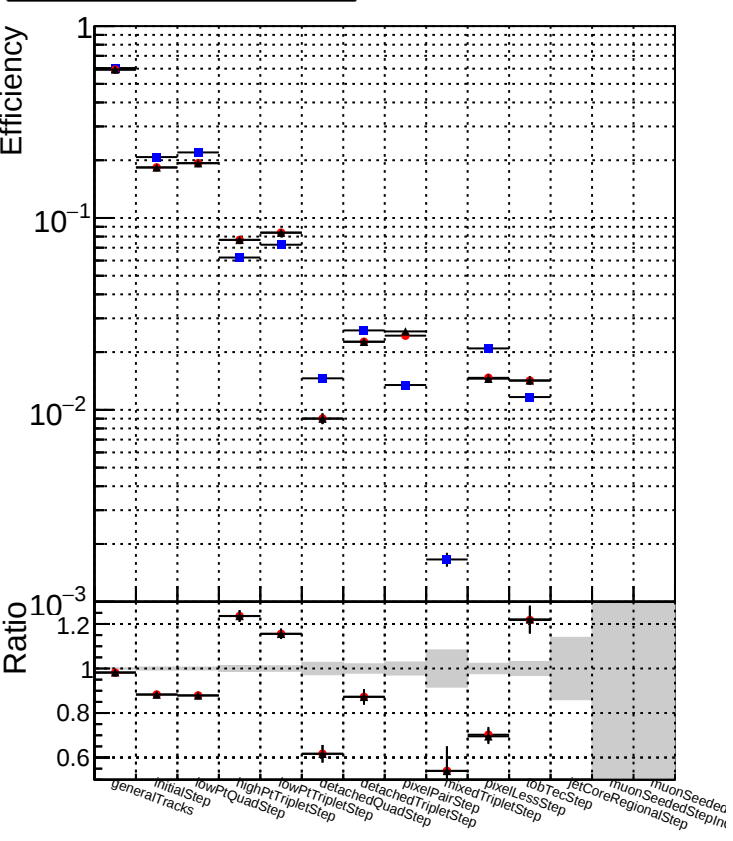
DQM_TT_original DQM_TT_originalCustomized DQM_TT_nocutCustomized
