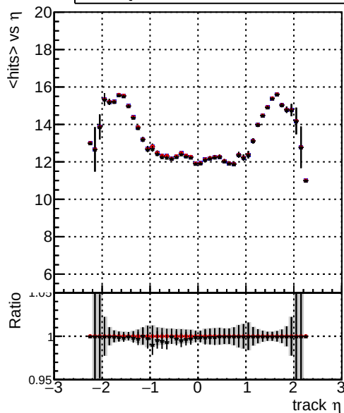
mean hits vs \eta — DQM_TT_original — DQM_TT_originalCustomized — DQM_TT_nocutCustomized
