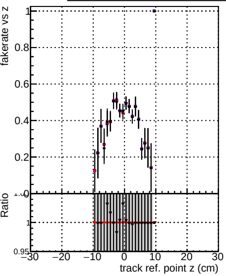
Fake rate vs verpos Legend: DOM TT original DOM TT originalCustomized DOM TT noCutCustomized
