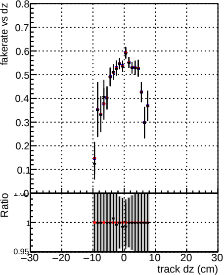
Fake rate vs dz Legend TT original Customized Blue line with dots TT original Customized Red line with dots TT original Customized Black line with dots TT original Customized
