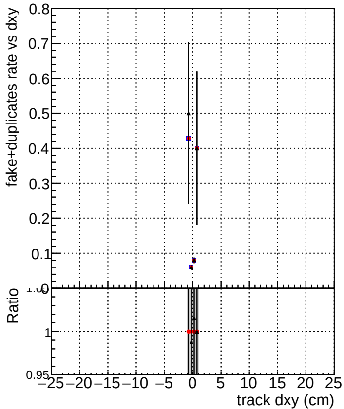
DQM_TT_original DQM_TT_originalCustomized DQM_TT_nocutCustomized
