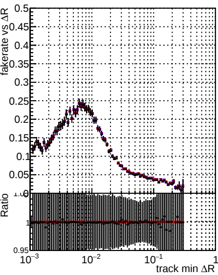
Fake rate vs \Delta R(\text{track, jet}) Legend: DQM TT original DQM TT originalCustomized DQM TT noCutCustomized
