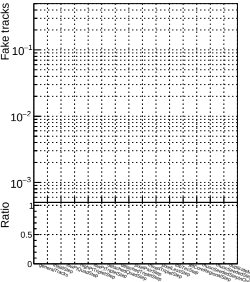
Number —●— DQM V0001 R000000001 Global mkFit batch2
