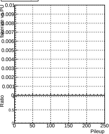
Fake rate vs Pileup
