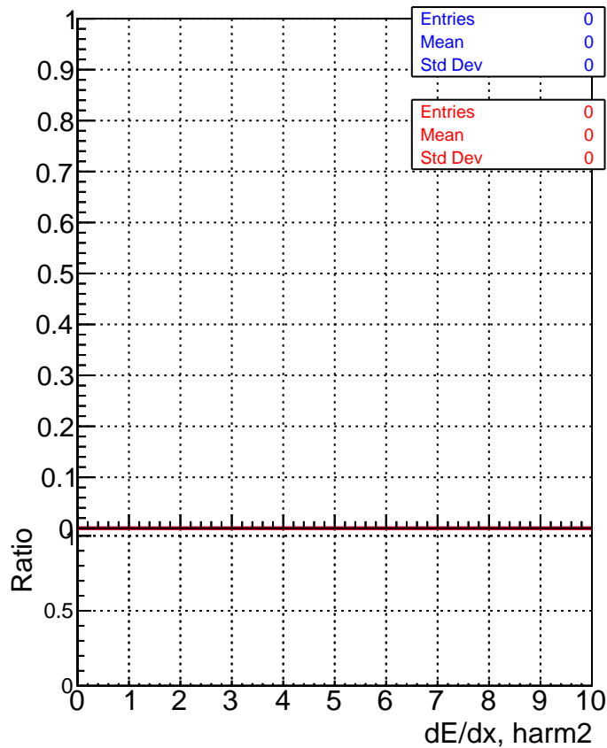
█ DQM_V0001_R000000001_Global_mkFit_batch3 █ DQM_V0001_R000000001_Global_mkFit_batch2
