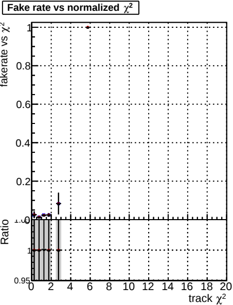
Fake rate vs. DOM TT original LooseNEW Loose3iter
