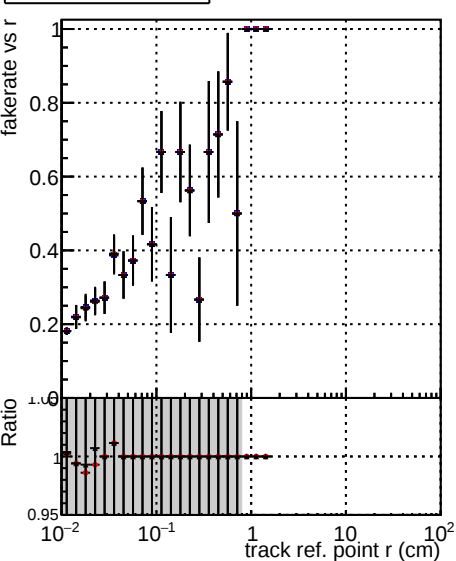
Fake rate vs v Legend: DOM TT original (black line with blue dots) DOM TT VLooseNEW (red line with red dots) DOM TT VLooseNEW3iter (black line with black dots)
