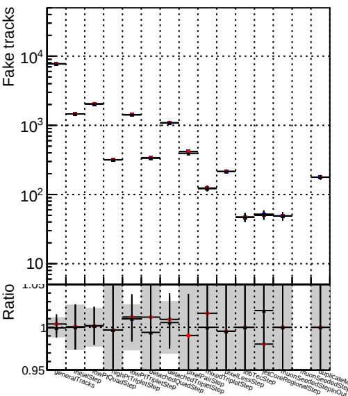
Number Model 1 DQM_TT_VLooseNEW 2 DQM_TT_VLooseNEW3iter
