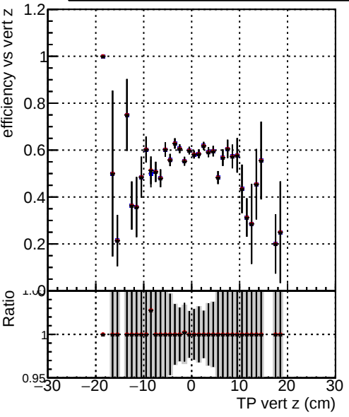
Efficiency vs vert z Legend: DQM_TT_original (blue line with circles) DQM_TT_VLooseNEW (red line with circles) DQM_TT_VLooseNEW3iter (black line with circles)
