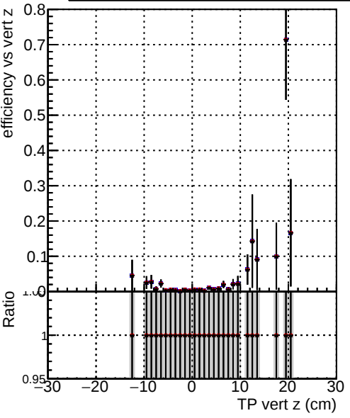
Efficiency vs TP vert z (cm) Legend: DQM_TT_original DQM_TT_VLooseNEW DQM_TT_VLooseNEW3iter
