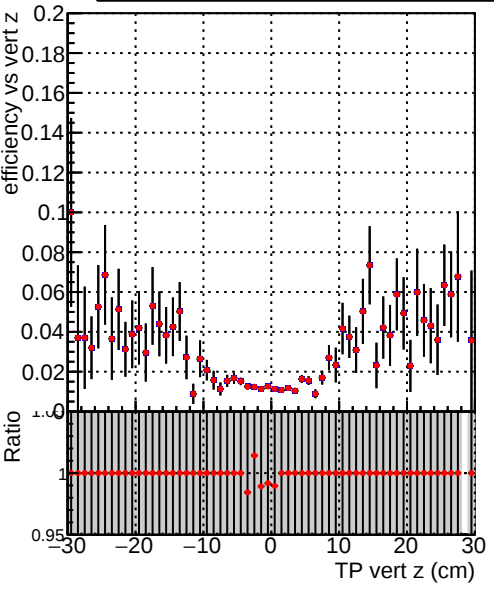
Efficiency vs TP vert z (cm) Legend: DQM_TT_original DQM_TT_cutopt-noSel
