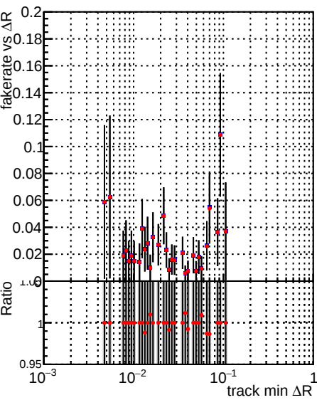
Fake rate vs ΔR(track, jet) DQM_TT_original DQM_TT_cutopt-noSel
