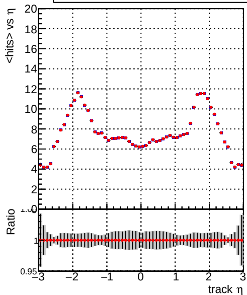
mean hits — DQM_TT__original — DQM_TT__cutopt-noSel
