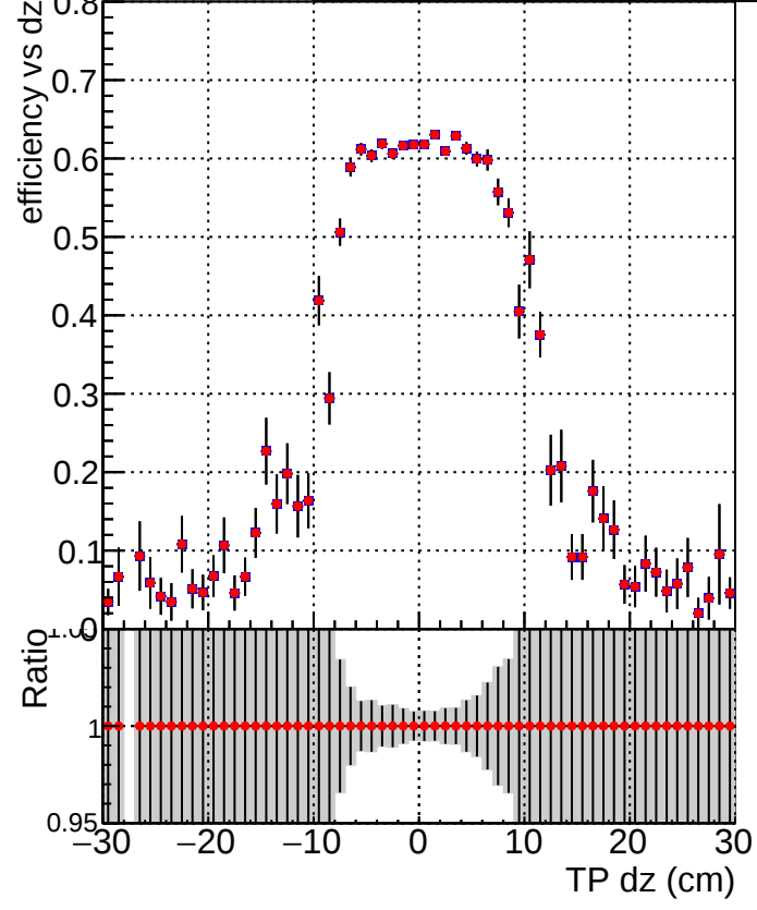
Efficiency vs Dz Legend: DQM_V0001_R0000000001_Global_mkFit_batchNO DQM_V0001_R0000000001_Global_mkFit_batch16
