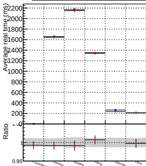
Average —●— DOM V0001 R0000000001 Global mkFit batch16
